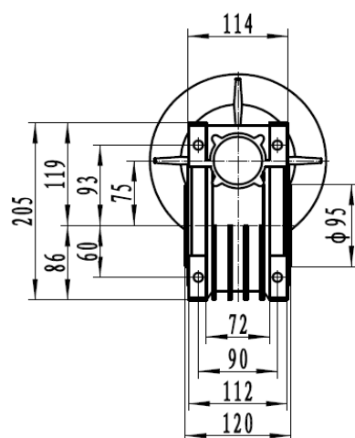
Output shaft hole
